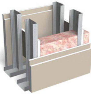
Partition Type 1
